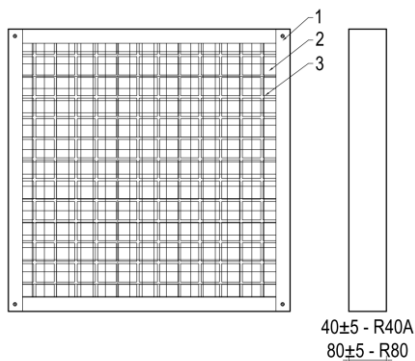
Fig. 1. Rectangular grille R40A, R80
