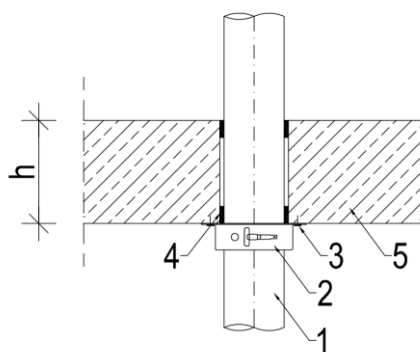
Fig. 3. Floor penetration
