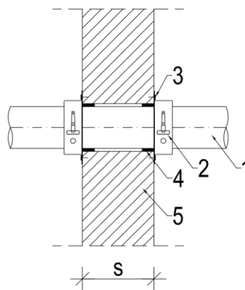
Fig. 2. Wall penetration
