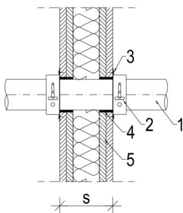
Fig. 1. Wall penetration
